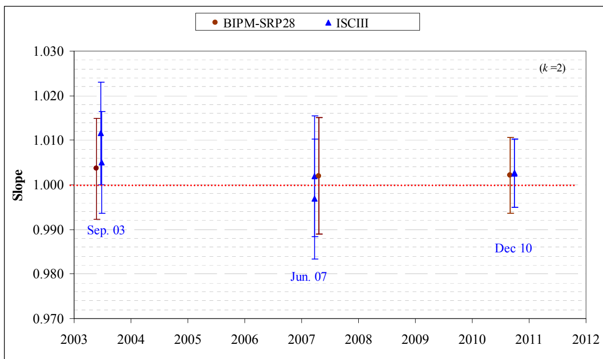
Figure 2 : Results of previous comparisons between SRP27, SRP28 and ISCI-III-SRP22 realised at the BIPM. Uncertainties are calculated at k = 2 , with the uncertainty budget in use at the time of each comparison.
